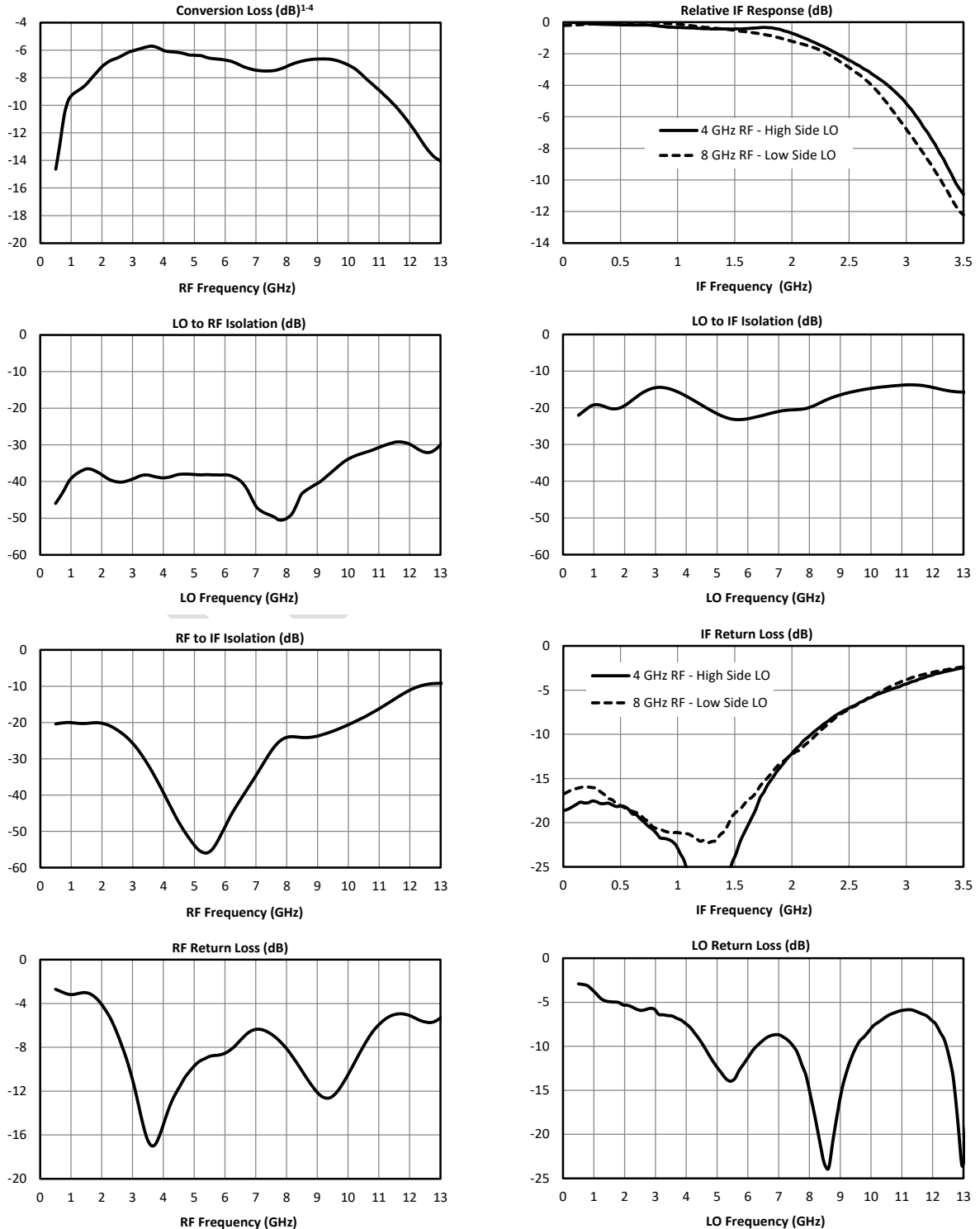
Typical Performance
